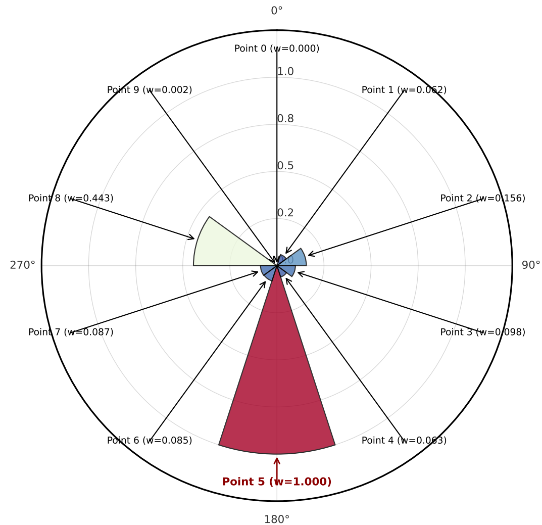
Attention Weights (MOA Task, Sample 100) Top Weight Point 5 ( w=1.0000 )
