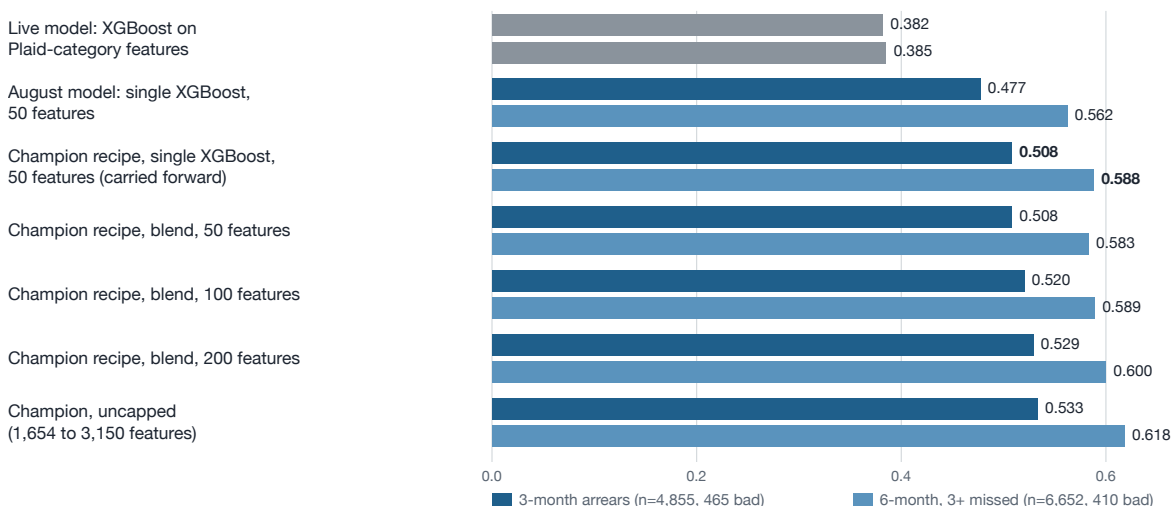
Figure 7. Out-of-time GINI: live model, August taxonomy model, and the champion at each feature cap
