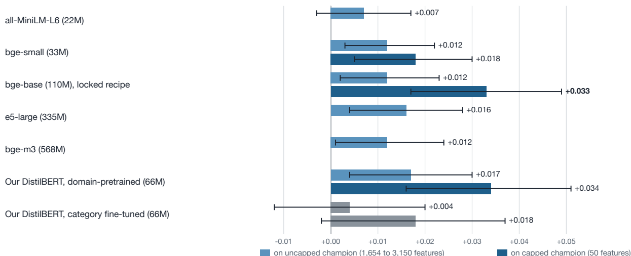
Figure 9. PR-AUC lift from one text score, on the uncapped and the 50-feature champion (95% CIs)
