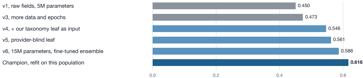
Figure 9. Sequence transformer versions against the champion, six-month GINI on 6,252 applicants
