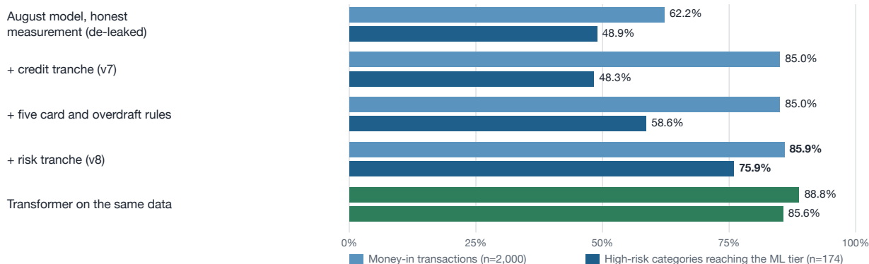
Figure 6. Linear classifier accuracy on the two September targets, step by step
