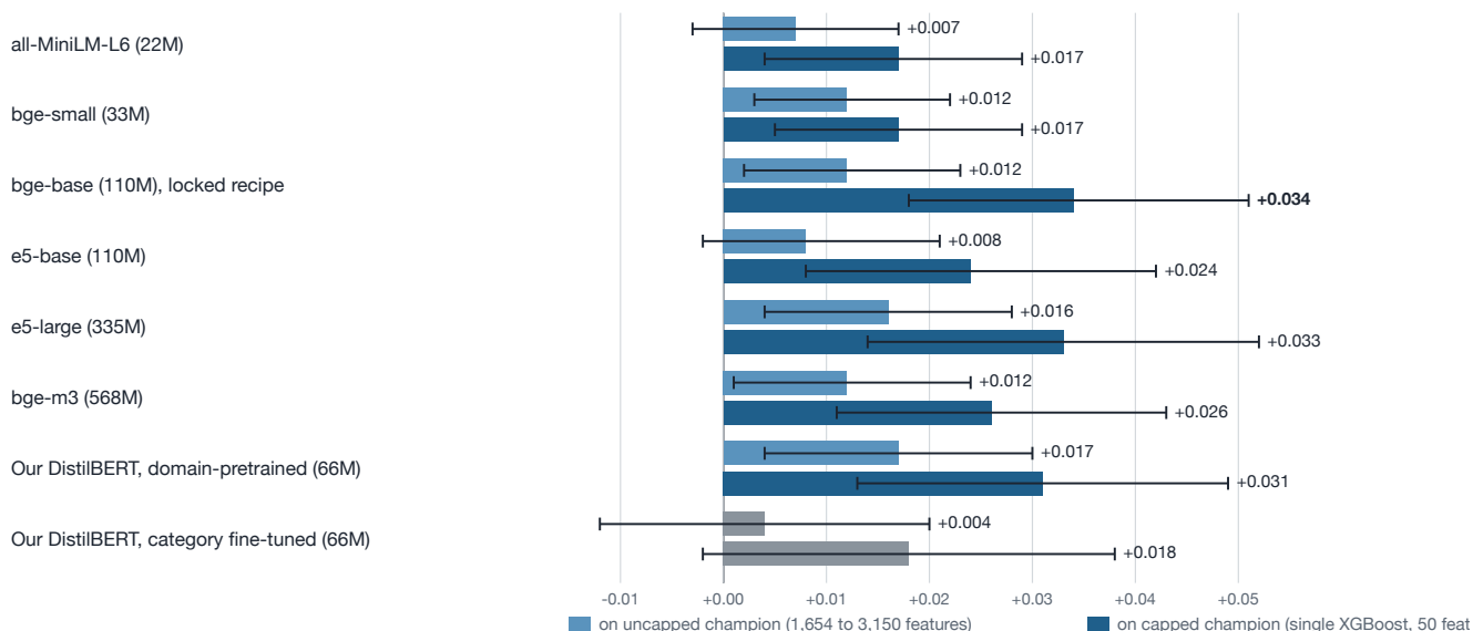
Figure 10. PR-AUC lift from one text score, on the uncapped and the 50-feature champion (95% CIs)
