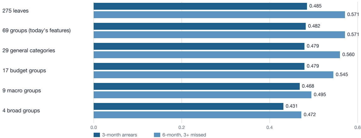
Figure 1. Risk-model GINI by number of category groups, August recipe (same cohort, same learner, 3 seeds)
