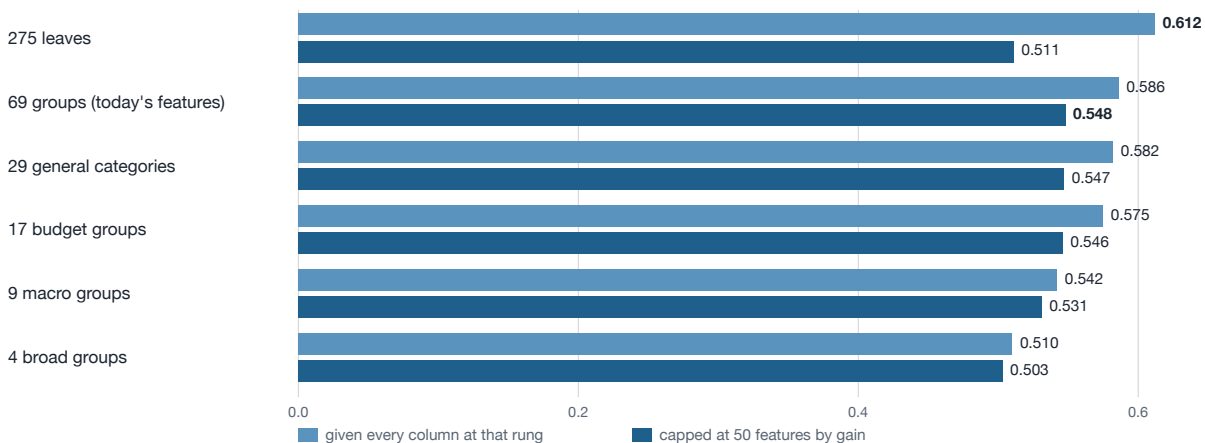
Figure 2. The same ladder with the champion recipe, six-month GINI, single XGBoost
