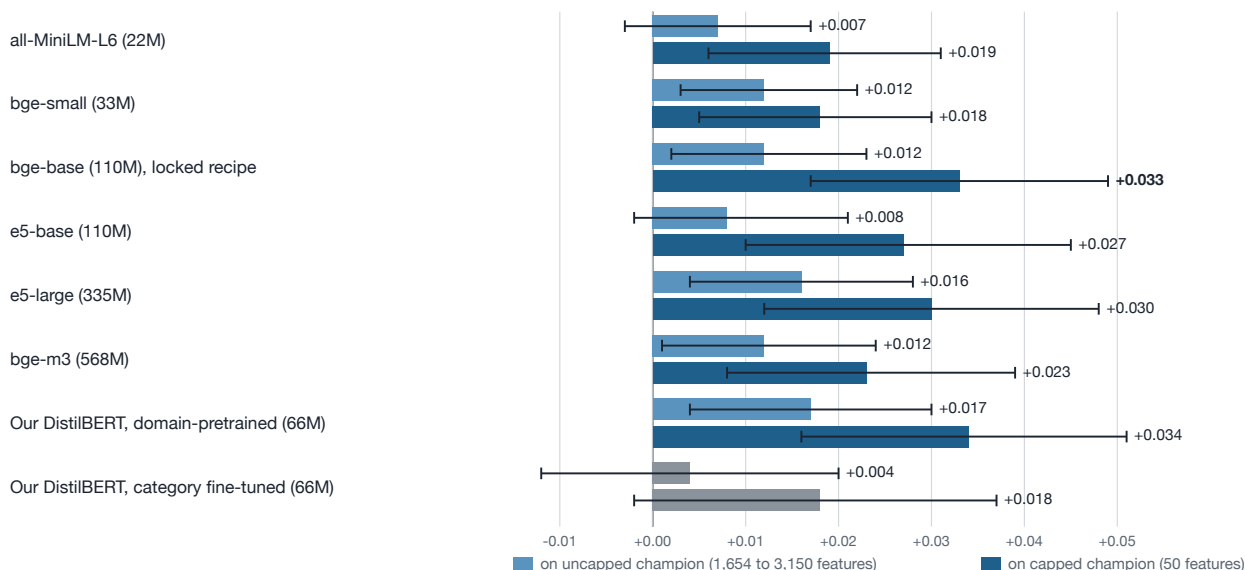
Figure 9. PR-AUC lift from one text score, on the uncapped and the 50-feature champion (95% CIs)
