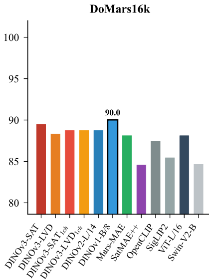
(b) Linear Probe
