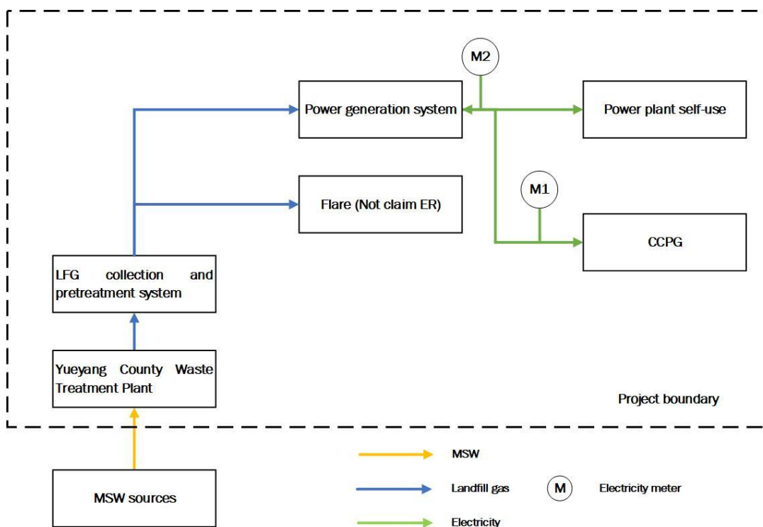
Figure 3.1 Diagram of the project boundary
