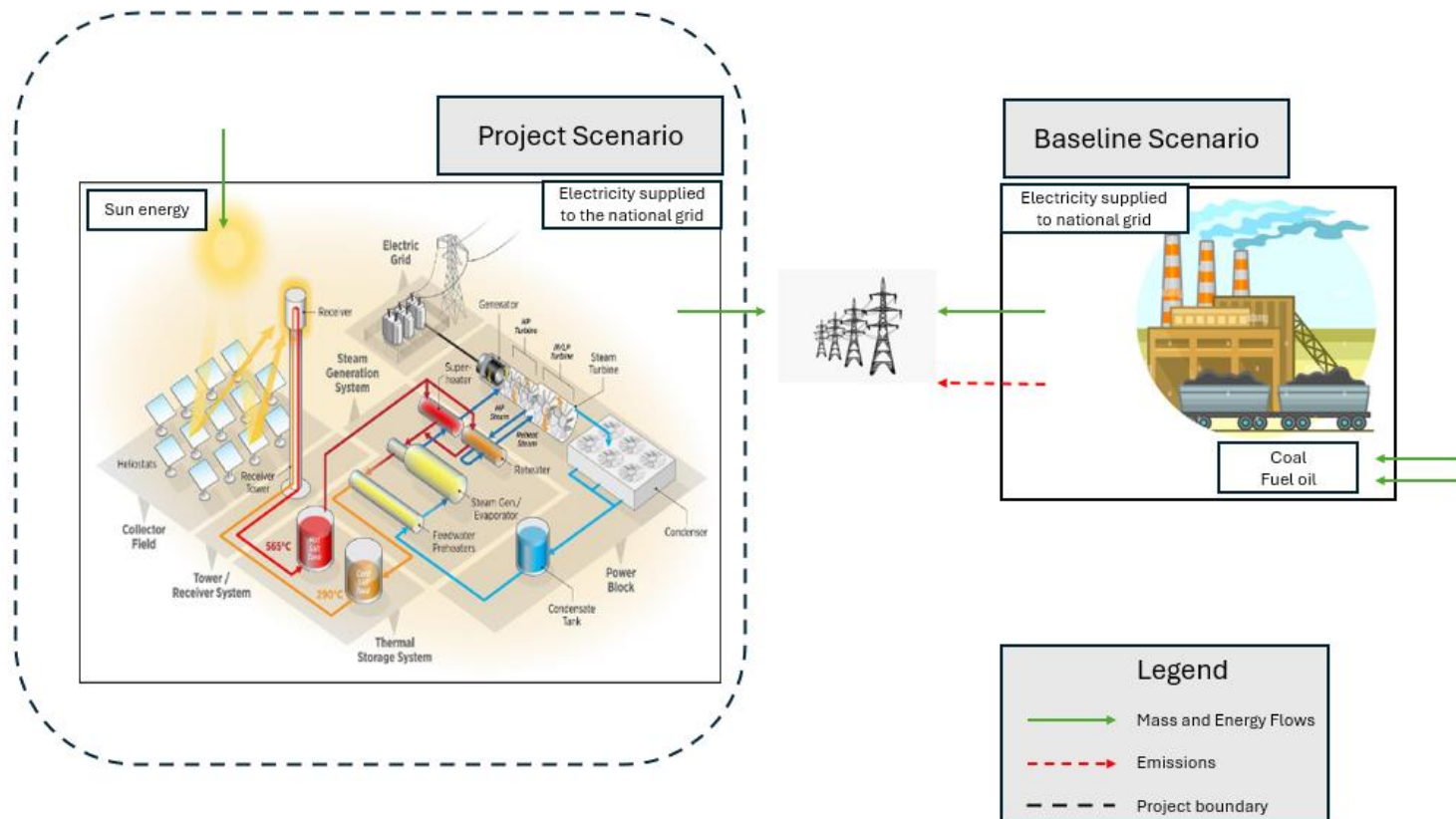
Figure 11: Project boundary, flows of mass and energy at Redstone CSP plant
