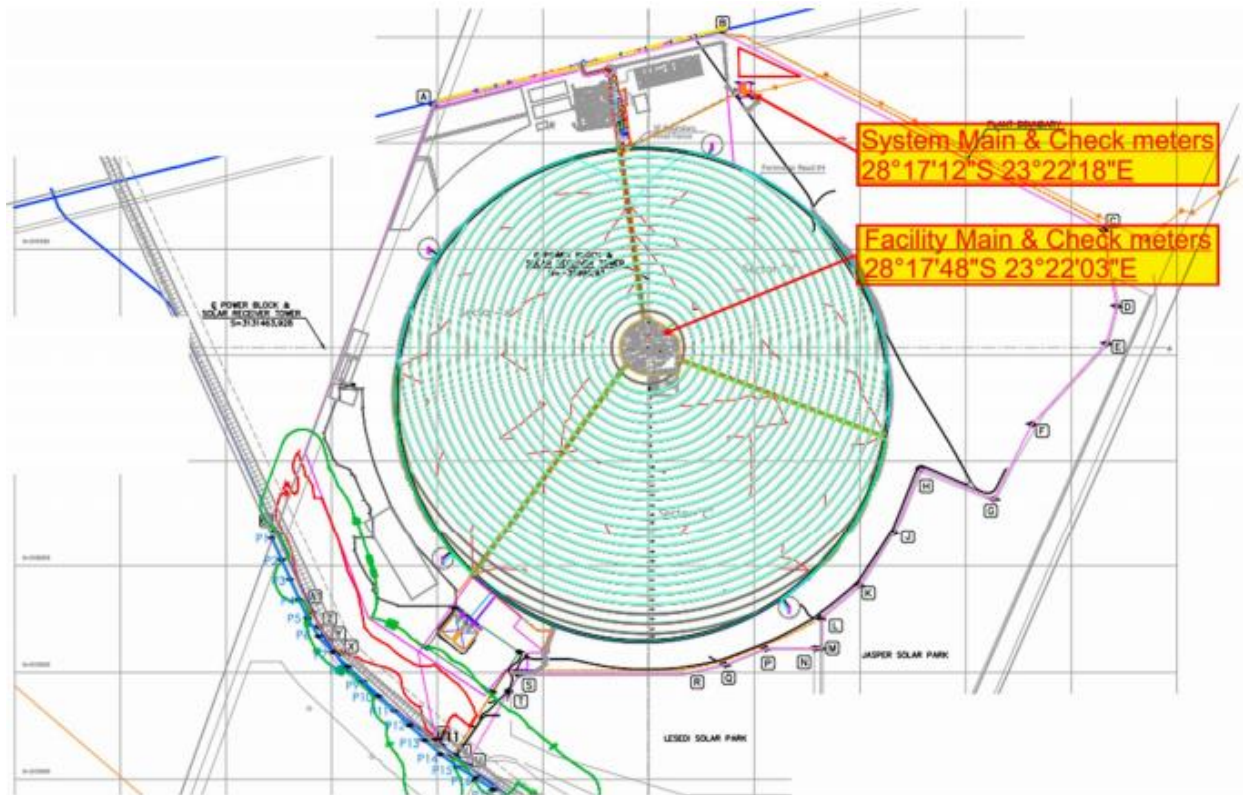
Figure 13: Meter locations on site
