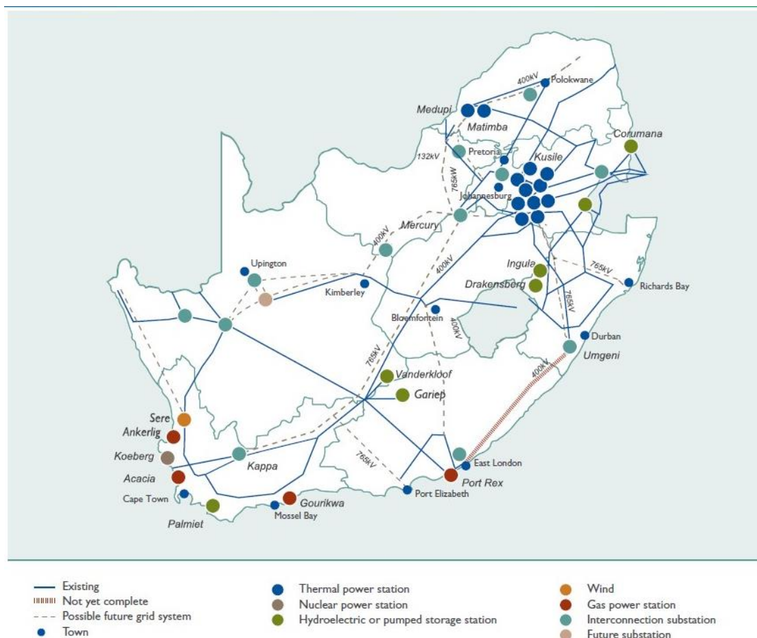
Figure 12: Project electricity system Source: [7]
