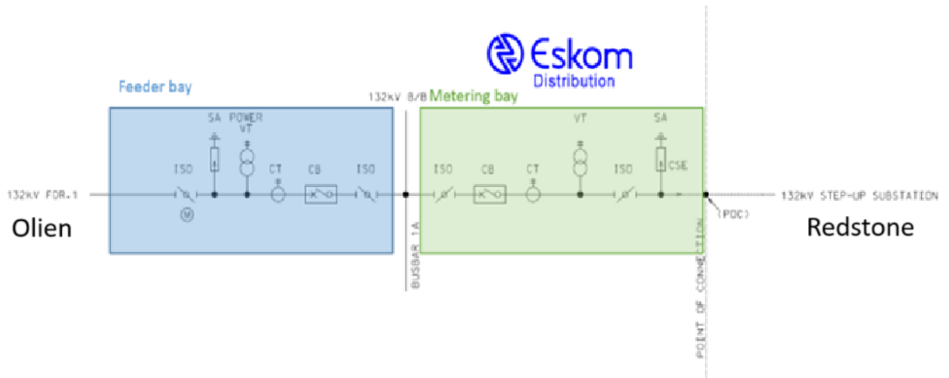
Figure 14: Single Line Diagram of meter configuration
