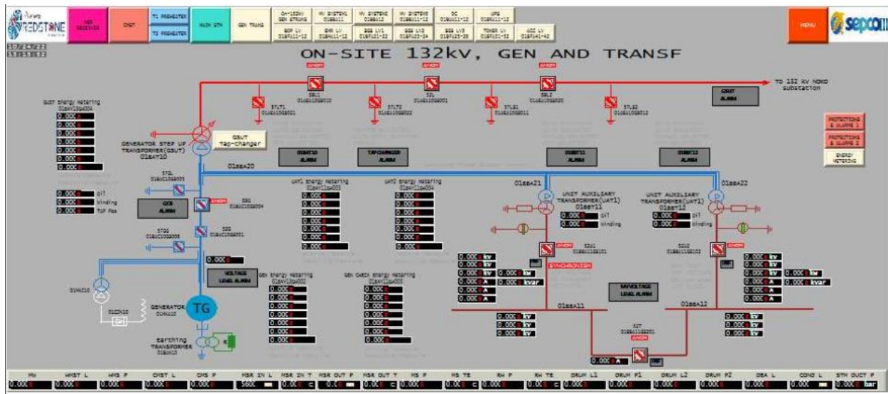
Figure 15: Indicative DCS screen for electricity generation and transfer
