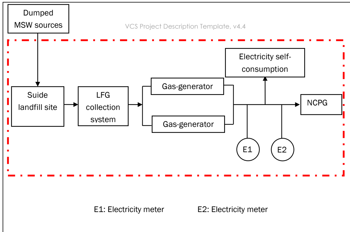
Figure 5.2 Monitoring system
