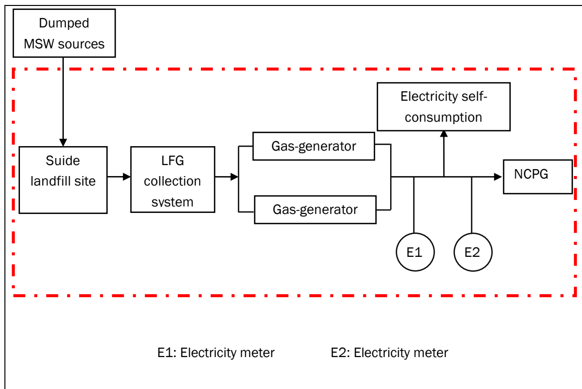
Figure 5.2 Monitoring system
