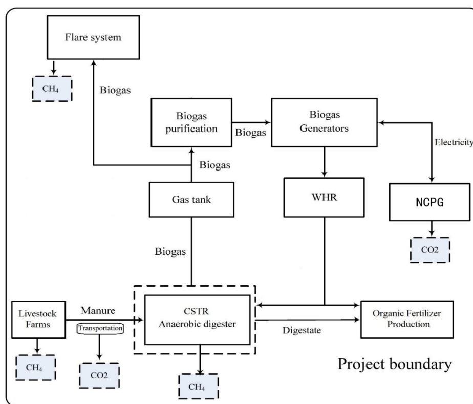
Figure 3-1 the project boundary of the Project Activity
