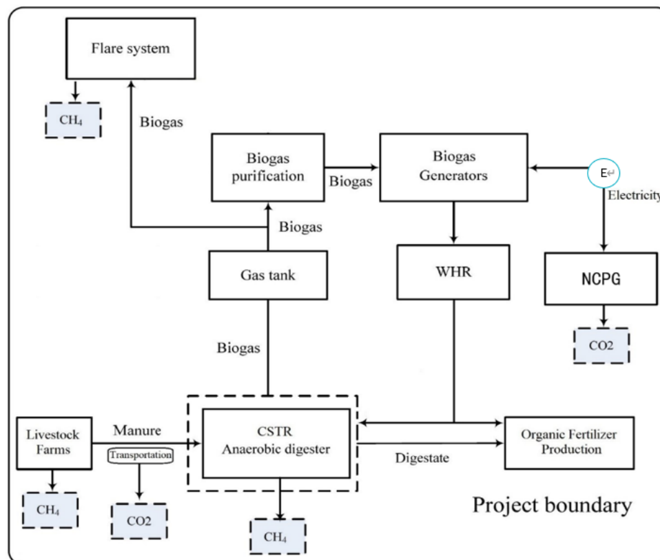
Figure 5-2 Project monitoring diagram
