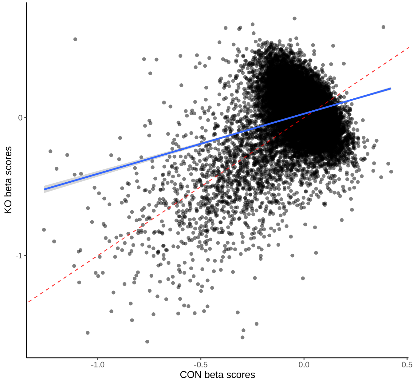
Comparison plot of non-normalised beta scores ?
