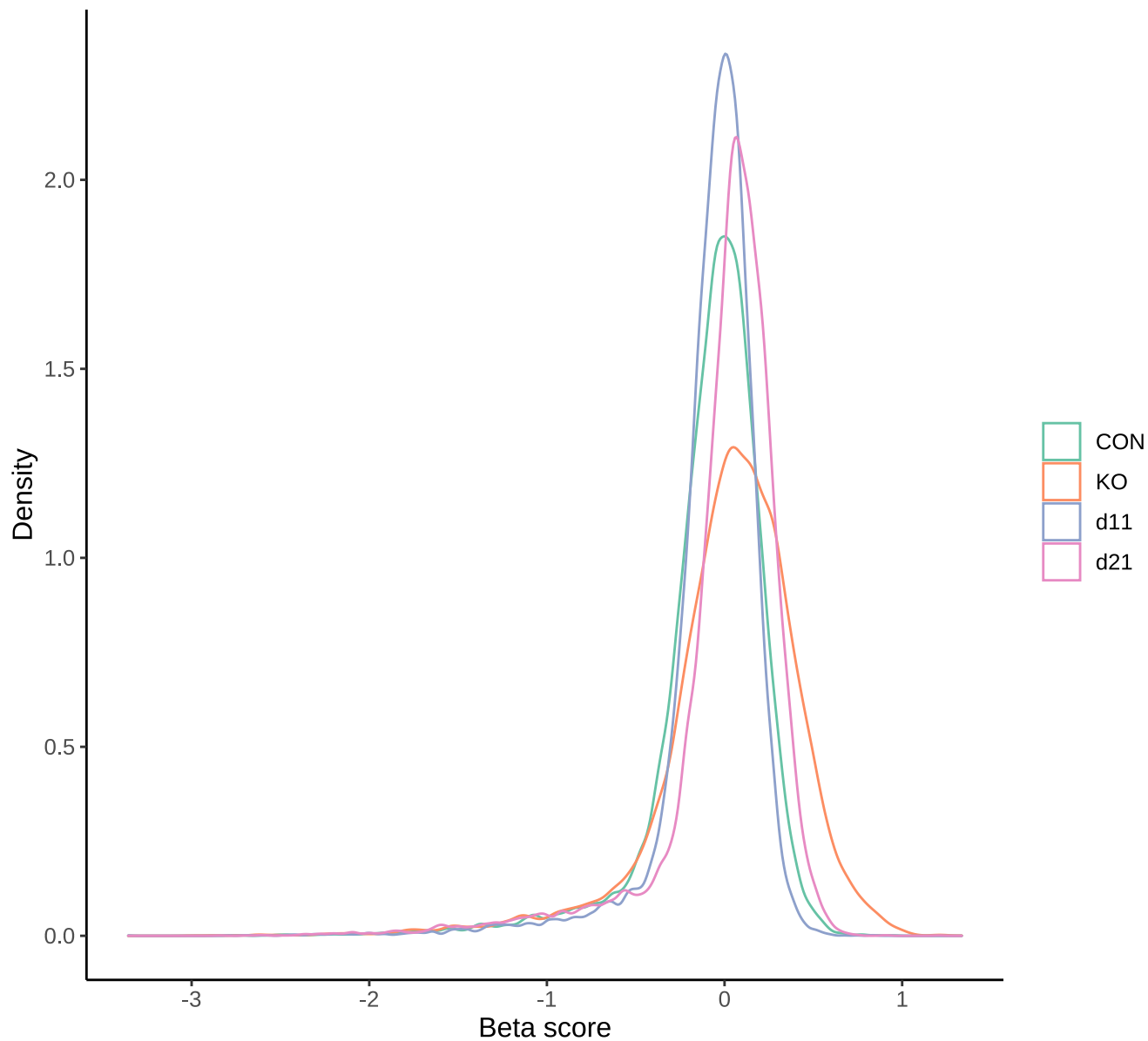
Density plot of normalised beta scores for all conditions shows normalisation
