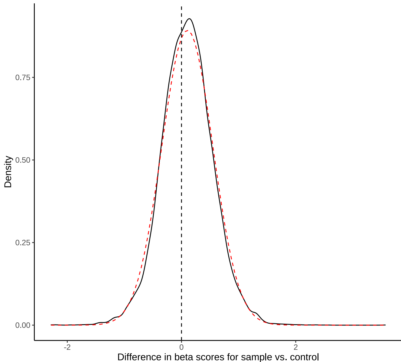
Distribution of deviation in normalised beta scores between CON vs. KO cells tends towards normal distribution
