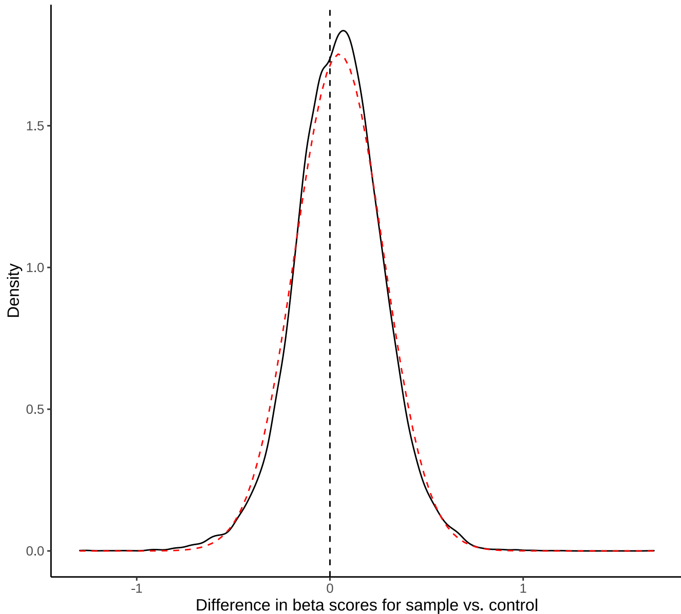
Distribution of deviation in non-normalised beta scores between CON vs. KO cells
