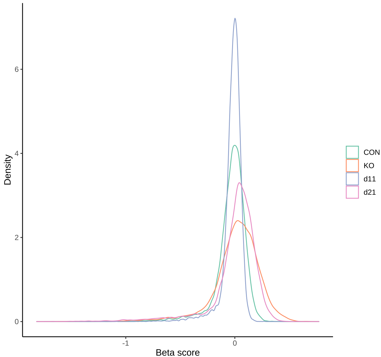
Density plot of non-normalised beta scores for all conditions
