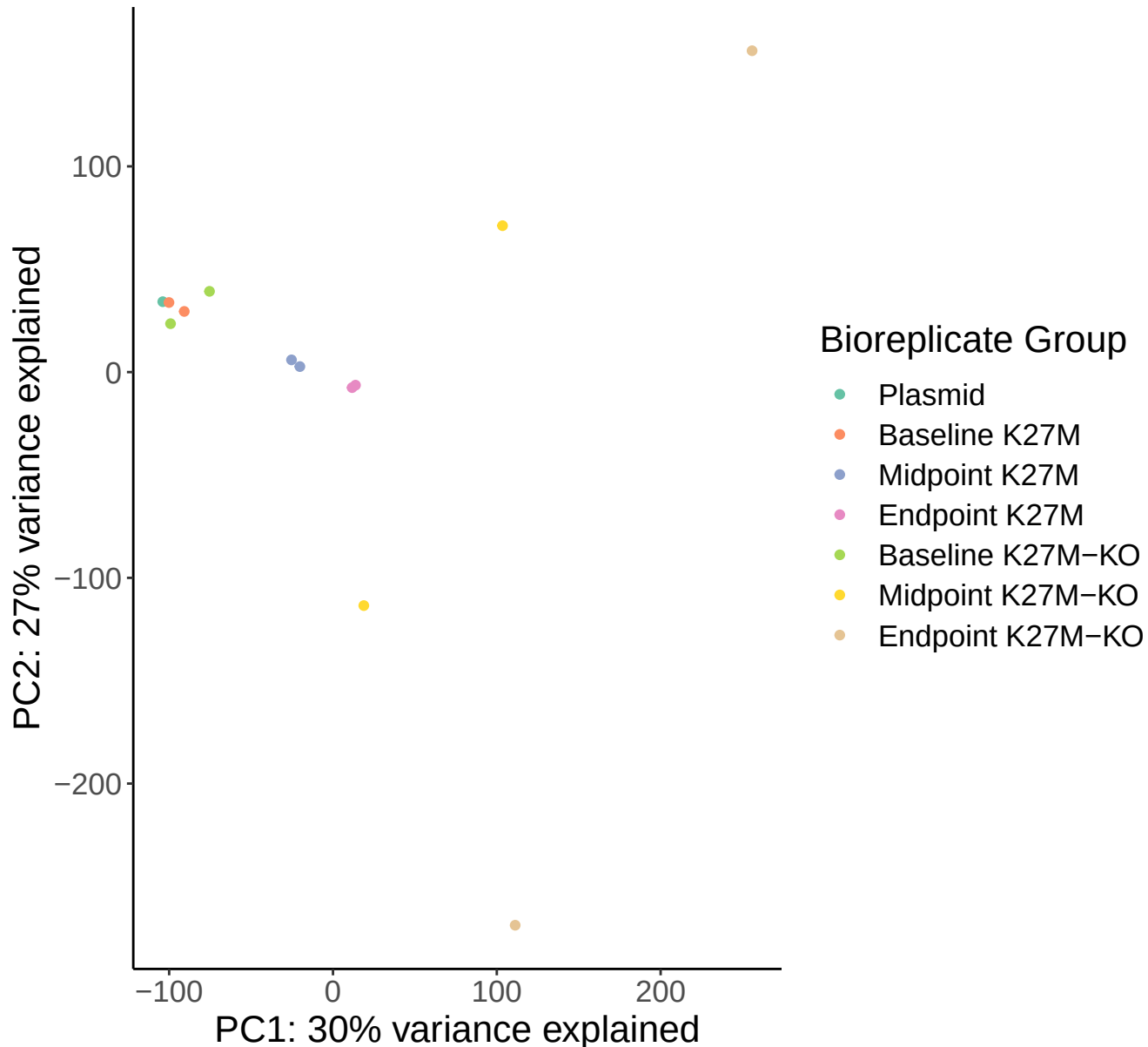
Biplot of principal components PC1 and PC2 shows v clustering of replicates
