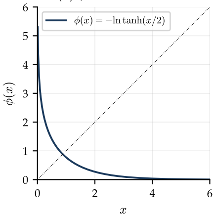
(a) \phi is its own inverse
