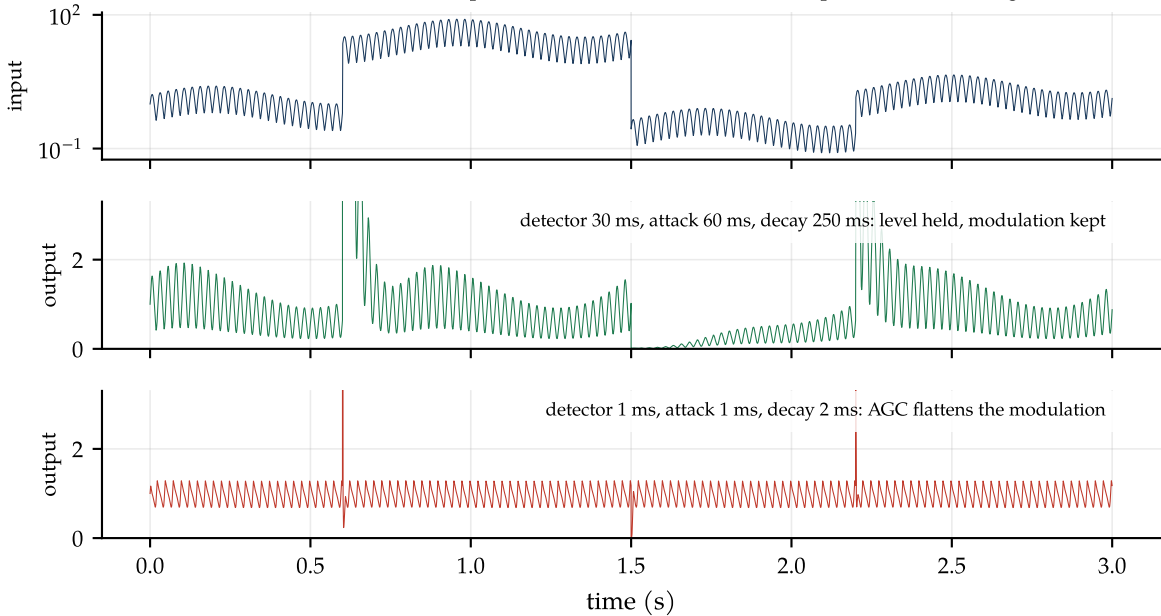
AGC on an AM envelope: +30 dB, -40 dB and +15 dB steps with slow fading
