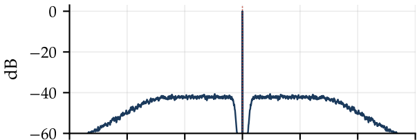
AM (DSB with carrier), \mu=0.8
