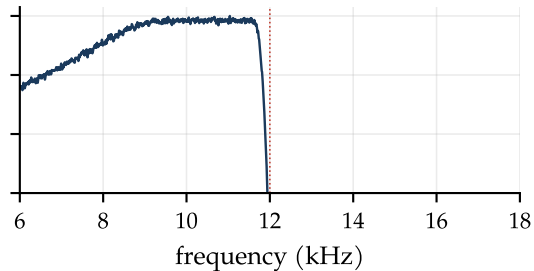
SSB, lower sideband
