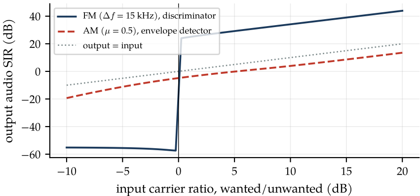
The capture effect (simulation, 500 Hz carrier offset)
