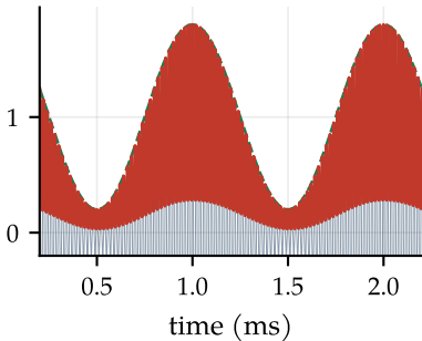
RC = 8 \mu\text{s} : too short (ripple)
