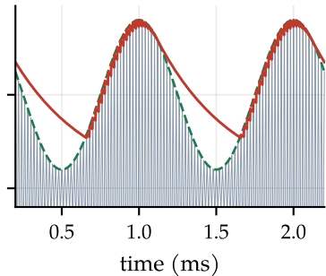
RC = 500 \mu\text{s} : diagonal clipping
