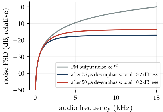
Effect on the parabolic noise, W = 15 kHz
