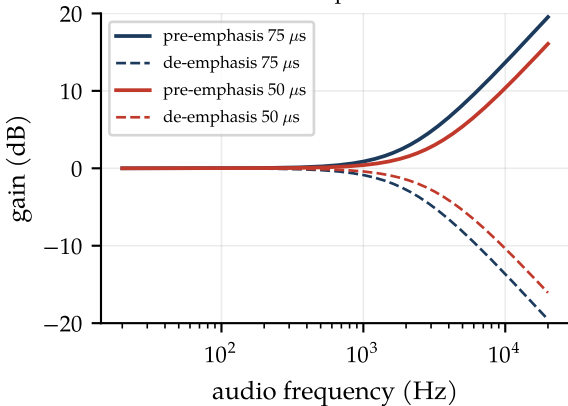
Broadcast emphasis curves
