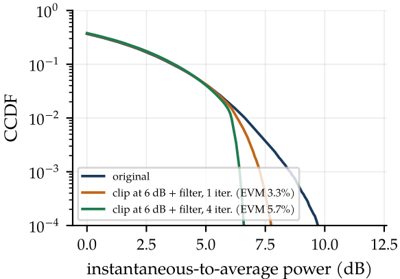
crest-factor reduction
