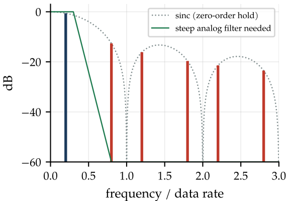
DAC at the data rate
