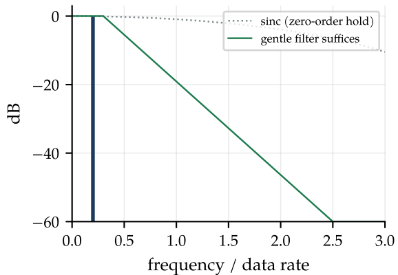
after 4\times digital interpolation
