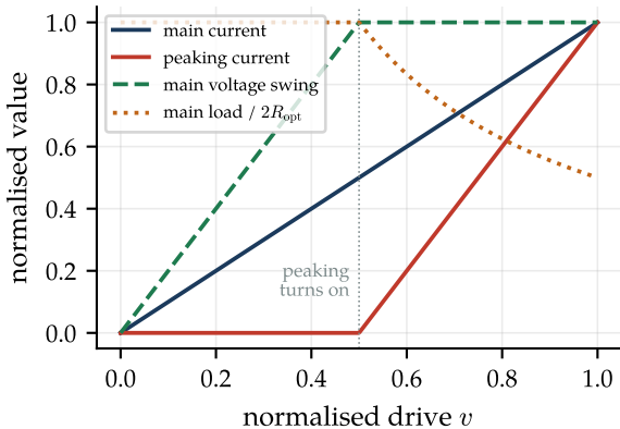
load modulation in a symmetric Doherty
