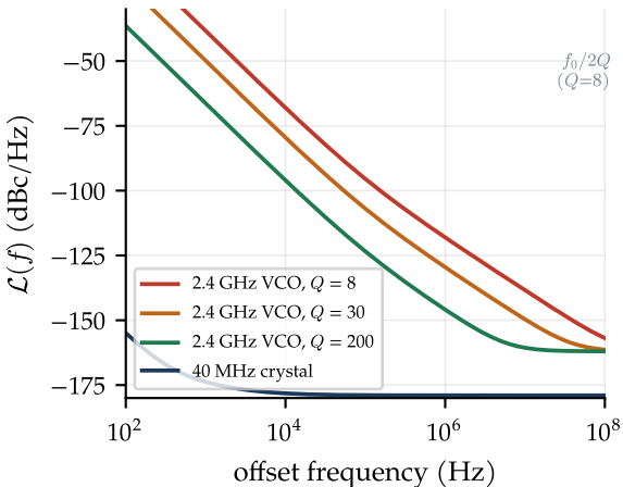
Leeson's model
