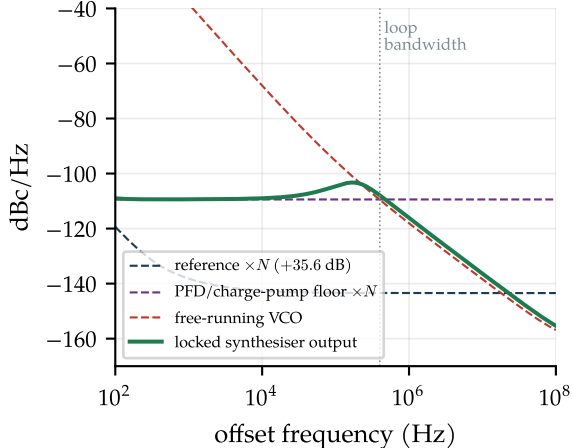
2.4 GHz PLL, N = 60 , f_{\text{ref}} = 40 MHz
