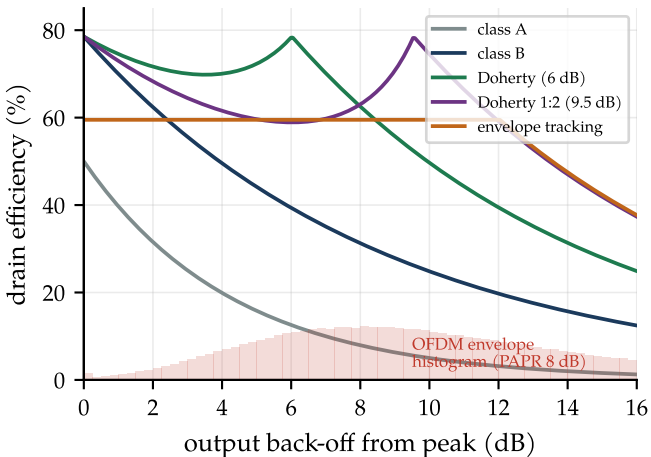
ideal efficiency versus back-off
