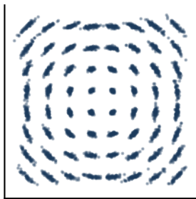
64-QAM, 3^\circ rms phase jitter
