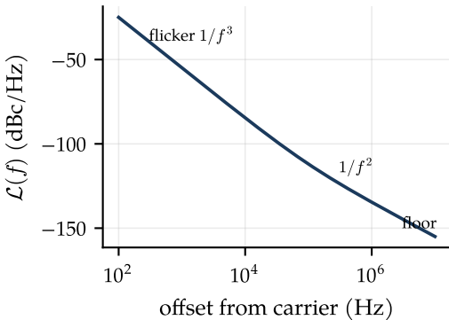
oscillator phase noise
