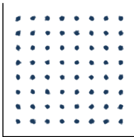
64-QAM, 0.5^\circ rms phase jitter
