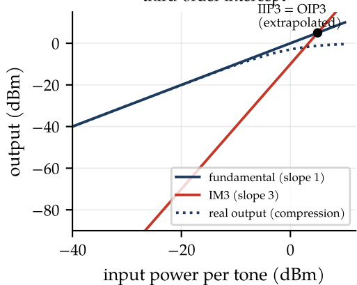
third-order intercept
