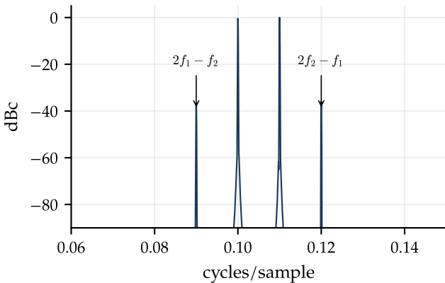
two-tone test: third-order products
