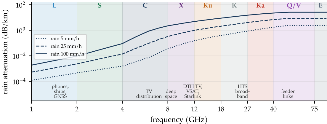
The satellite bands: more bandwidth upstairs, more rain too
