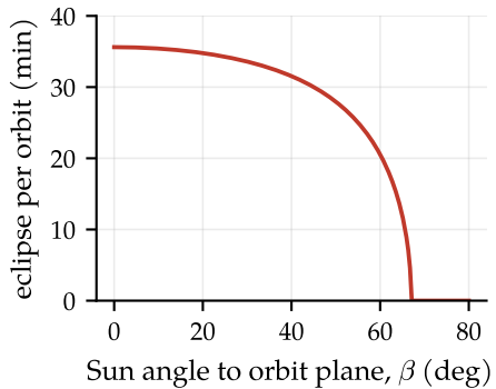
LEO 550 km: most orbits
