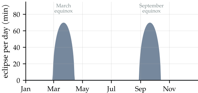
GEO: two eclipse seasons a year
