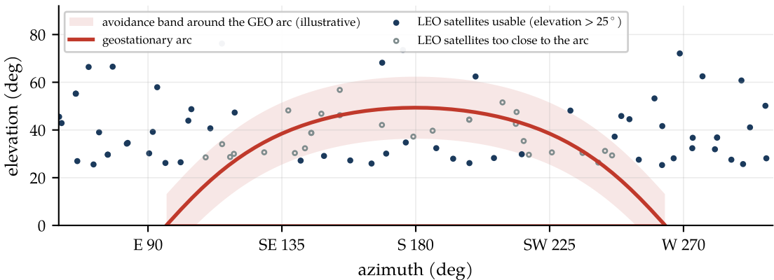
The southern sky seen from 35° N: where a LEO terminal may and may not look
