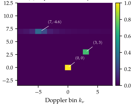
(b) response to one DD symbol
