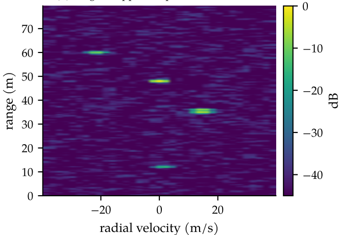
(a) range--Doppler map, 28 GHz, 396 MHz
