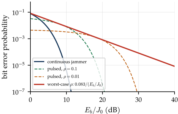
(a) DSSS-BPSK, pulsed jammer
