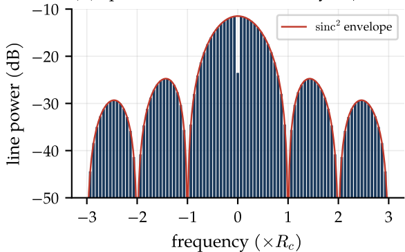
(b) spectrum, N = 15 : lines every R_c/N
