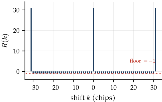
(a) periodic autocorrelation, N = 31
