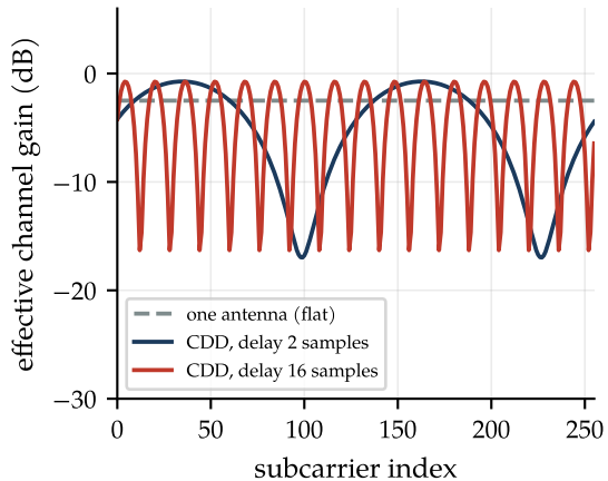
(b) cyclic delay diversity
