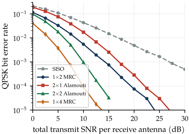
(a) Alamouti vs receive MRC
