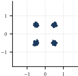
after the Alamouti combiner
