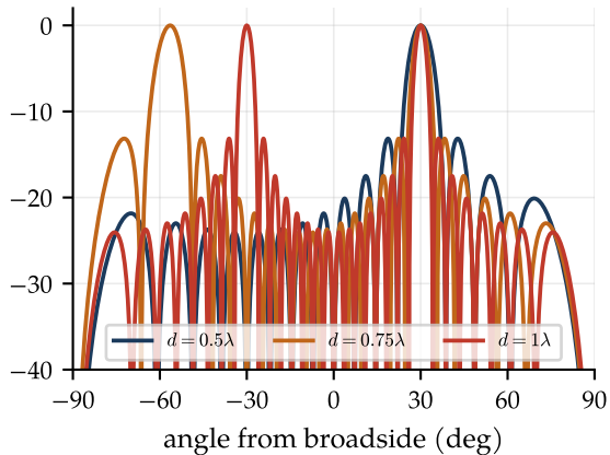
(b) steered to 30°: grating lobes
