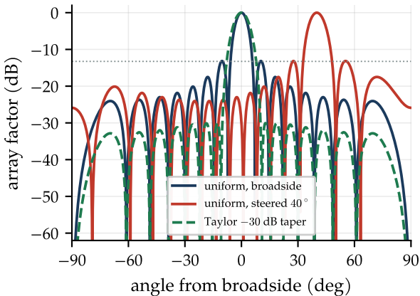
(a) 16 elements, d = \lambda/2
