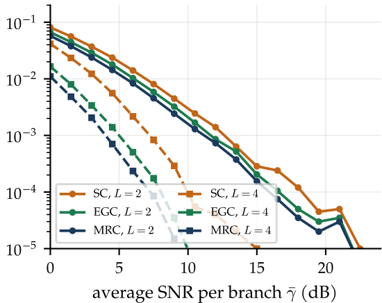
(b) selection vs equal-gain vs MRC
