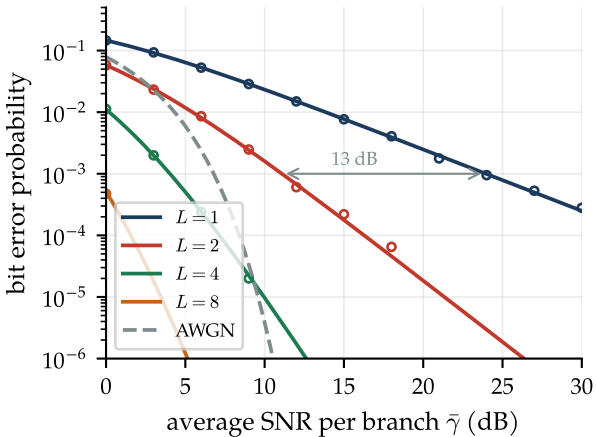
(a) BPSK with L -branch MRC
