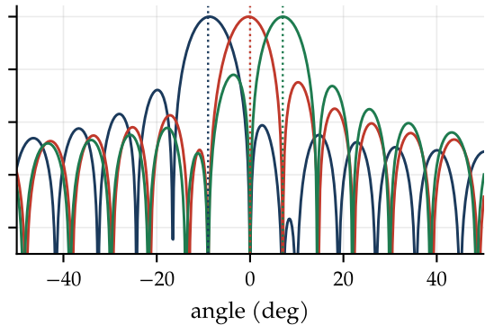
ZF precoding, M = 16 : nulls on the others
