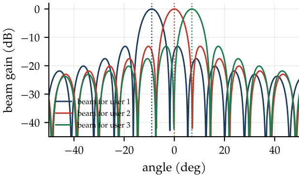
MR precoding, M = 16 : leaks onto neighbours
