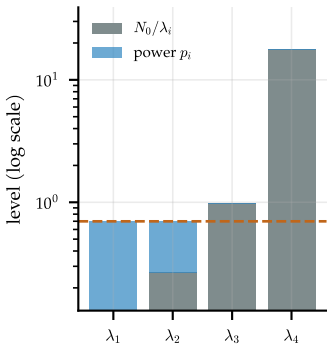
SNR 0 dB: 2 pipes used
