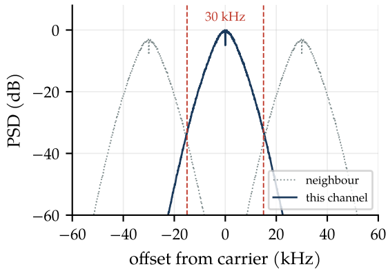
(b) simulated FM spectrum, 12 kHz dev.
