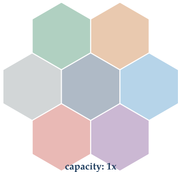
(a) R = 2 km: 7 cells
