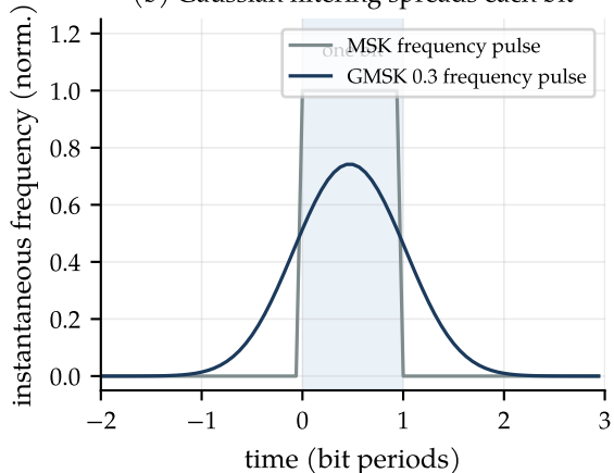
(b) Gaussian filtering spreads each bit
