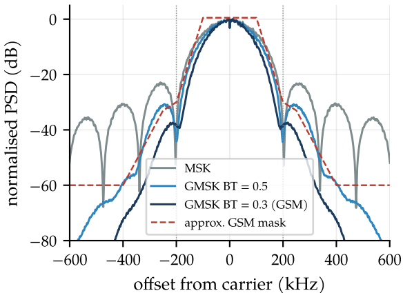
(a) Spectrum at 270.833 kb/s
