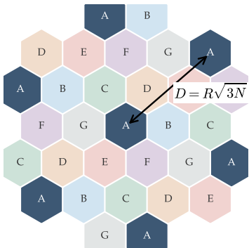
(a) N = 7 : co-channel cells (A)
