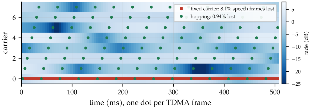
A walker at 3 km/h, 900 MHz: deep fades last ~100 ms (statistics from a 2-minute run)
