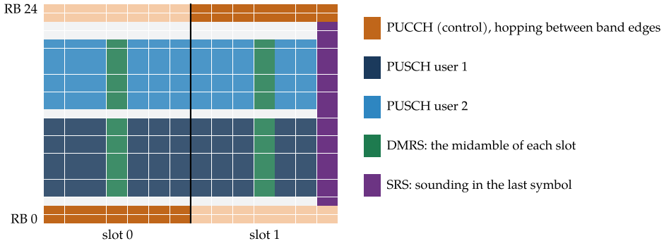
LTE uplink subframe, 5 MHz (illustrative allocation)
