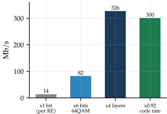
(b) from REs to ~300 Mb/s
