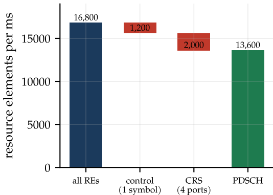
(a) 20 MHz: 100 RBs x 14 symbols
