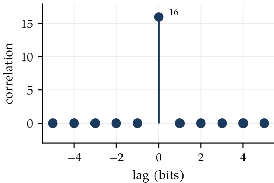
(a) TSC 0: ideal within \pm 5 bits
