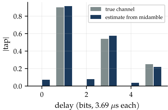
(b) one correlation = channel estimate
