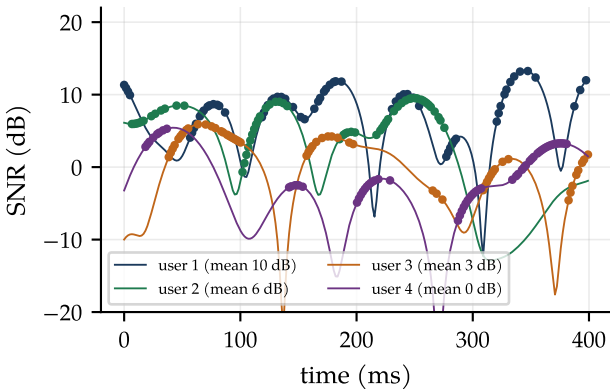
(a) dots: who the PF scheduler serves
