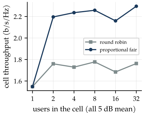
(b) multi-user diversity gain
