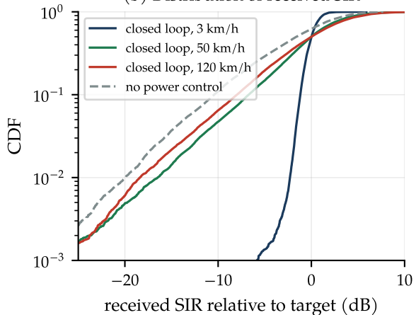
(b) Distribution of received SIR
