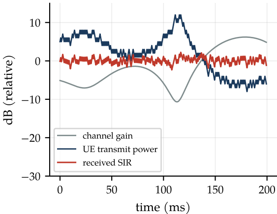
(a) 3 km/h, 1 dB steps every 0.667 ms
