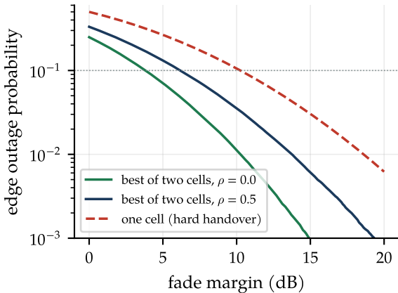
(a) Macrodiversity, shadowing \sigma = 8 dB
